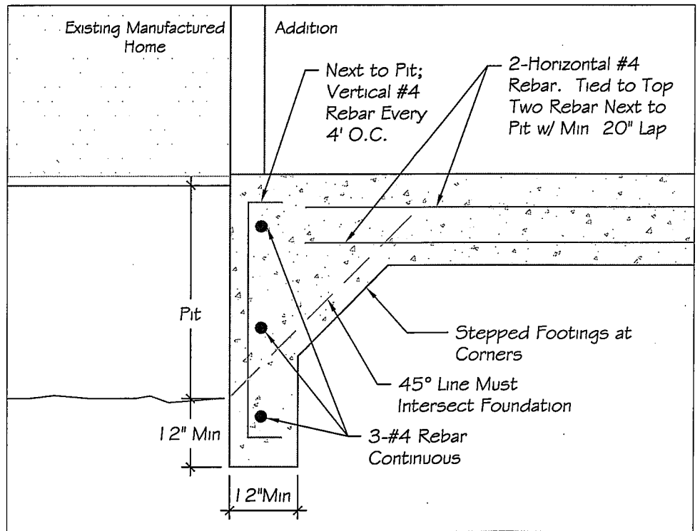
Section B-B
